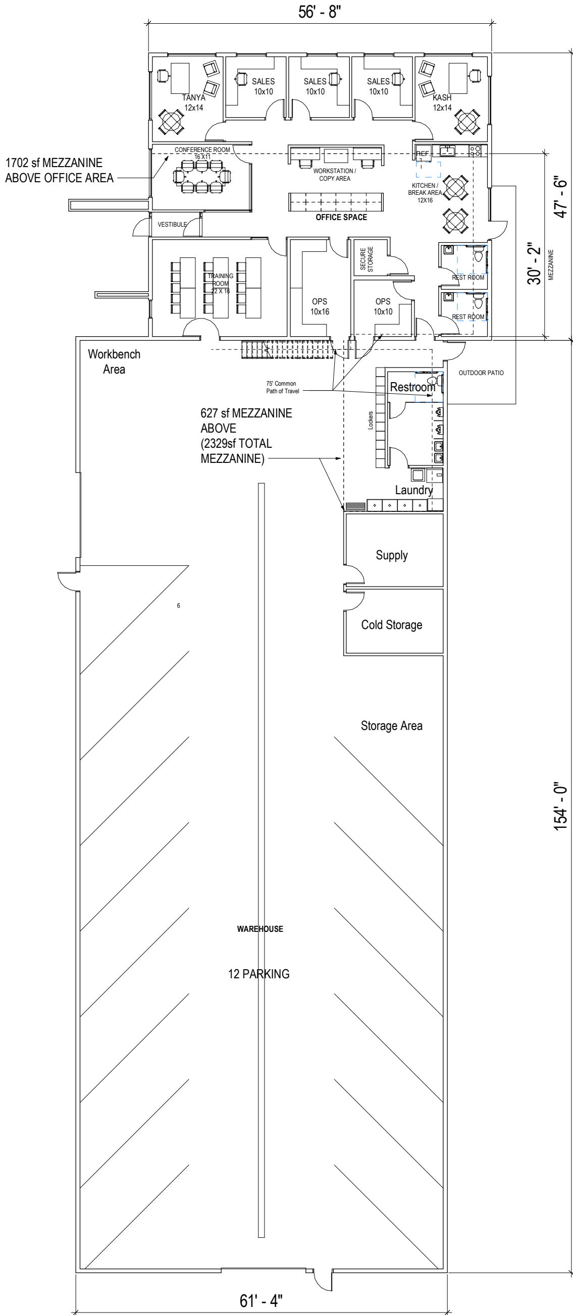
1 FIRST FLOOR PLAN 1/8" = 1'-0"
